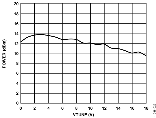
Figure 19. Output Power vs. Tuning Voltage with VDD = 3V
